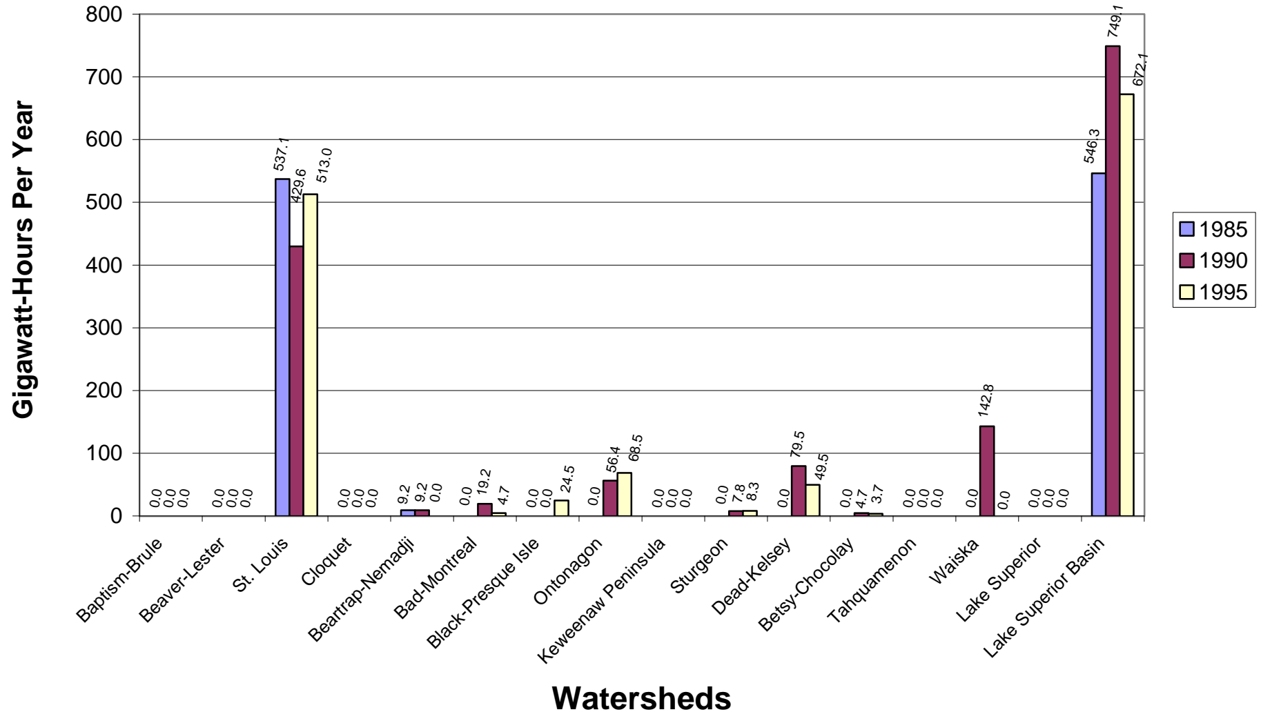
Fig. 4.16c. Hydroelectric Power Generation by Watershed U.S Lake Superior Basin
