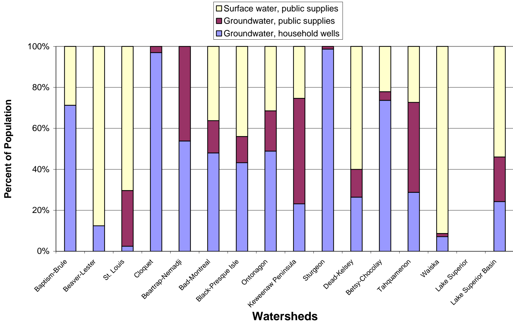
Fig. 4.18g. Percentage of Population Served by Groundwater and Surface Water Supplies, U.S. Lake Superior Basin, 1990
