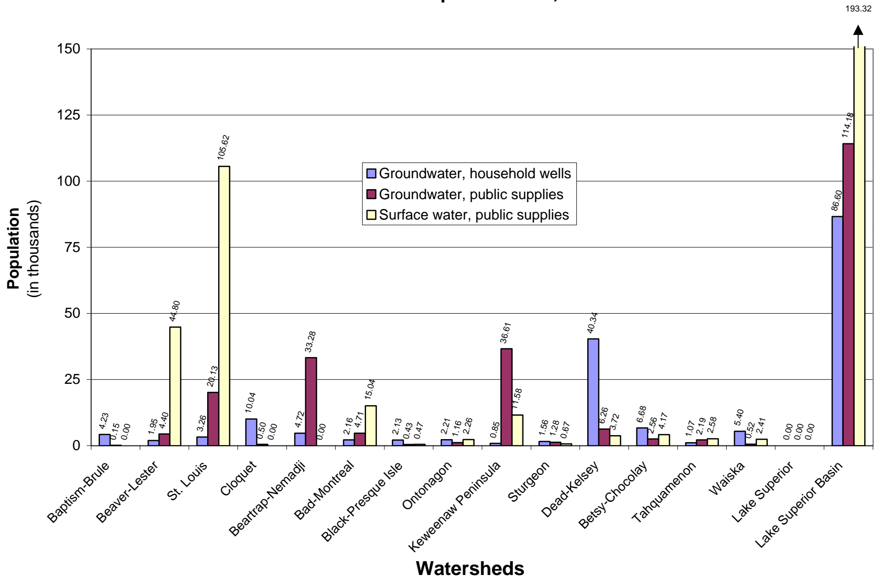
Fig. 4.18i. Population Served by Groundwater and Surface Water Supplies U.S. Lake Superior Basin, 1985
